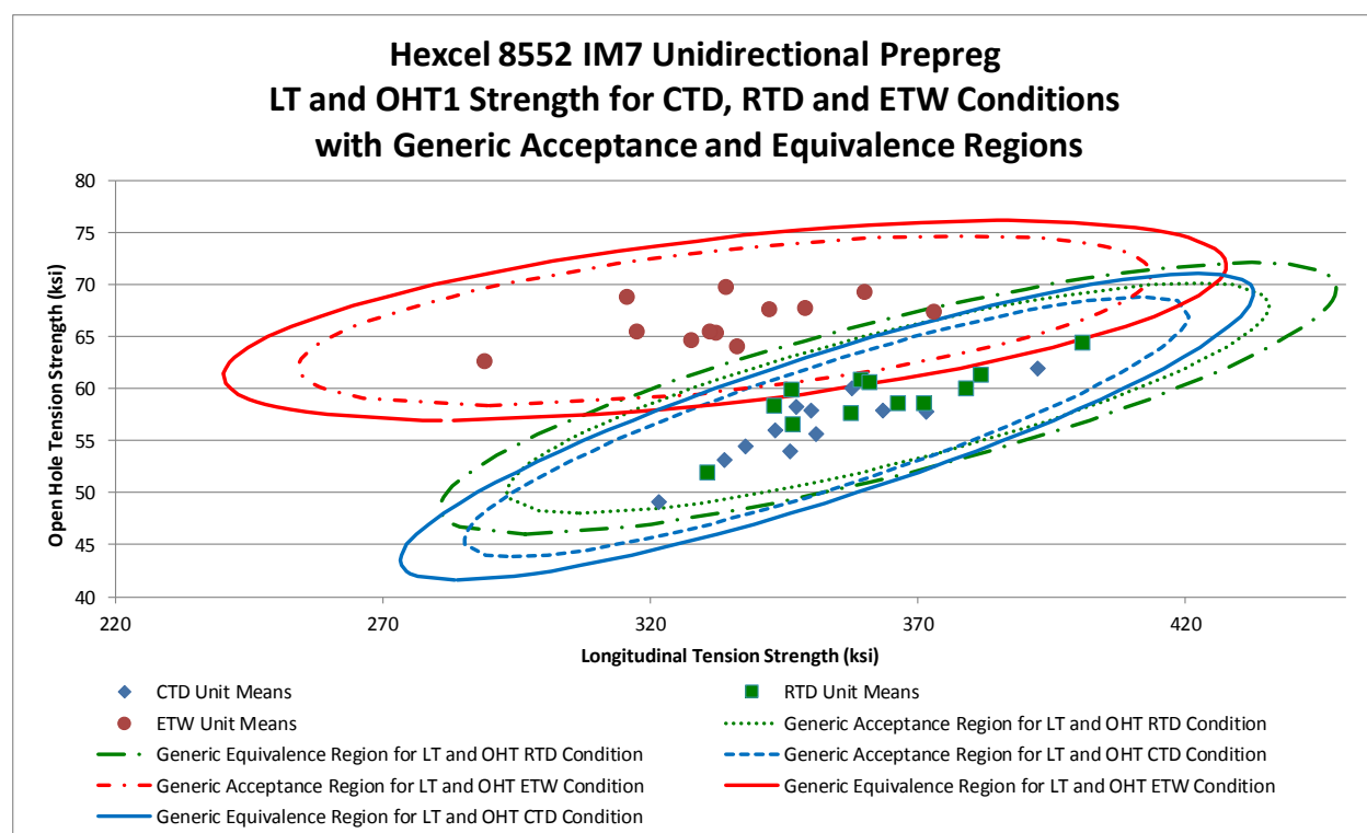
Figure 21: LT and OHT1 Strength CTD, RTD and ETW Conditions Acceptance and Equivalence Ellipses
