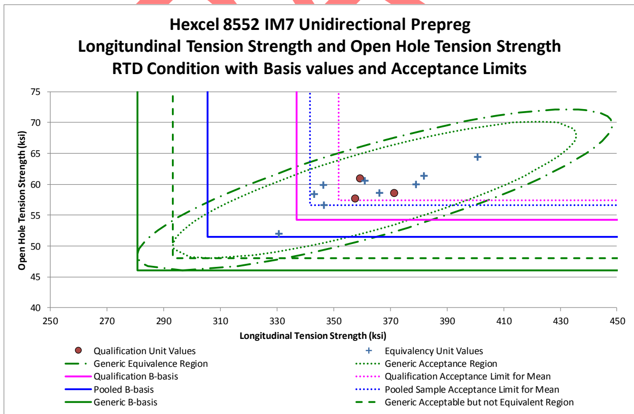
Figure 18: LT and OHT1 Strength RTD Conditions Acceptance and Equivalence Ellipses
