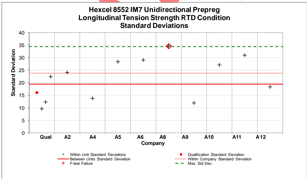
Figure 47: LT RTD Strength Standard Deviations by Company
